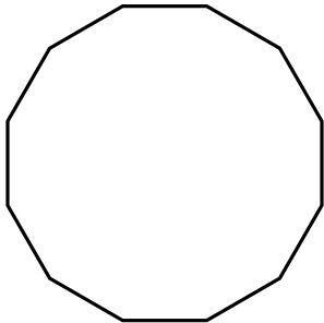
dodecagon
