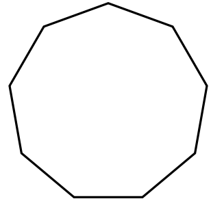
nonagon
