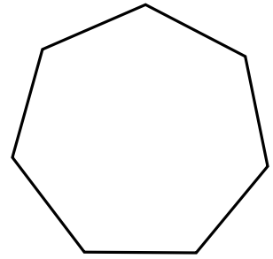
heptagon
