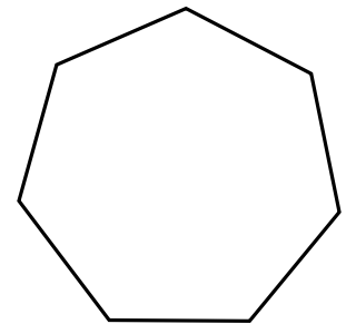
heptagon
