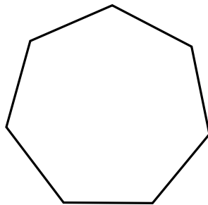
heptagon
