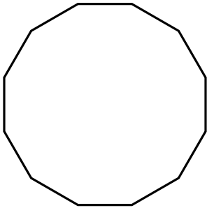
dodecagon
