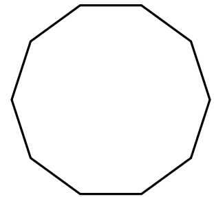
decagon
