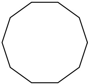
decagon
