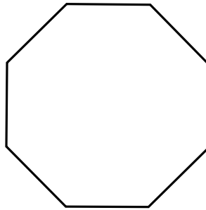
octagon
