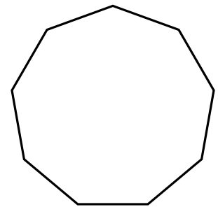
nonagon
