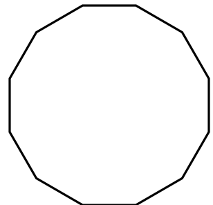
dodecagon
