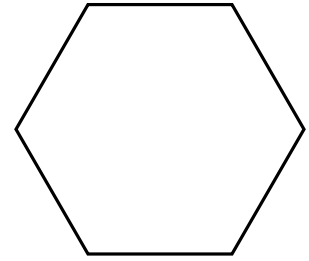
hexagon
