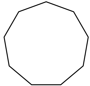
nonagon
