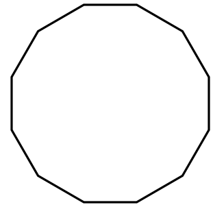
dodecagon
