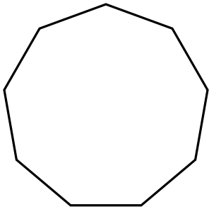
nonagon
