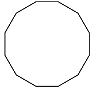
dodecagon
